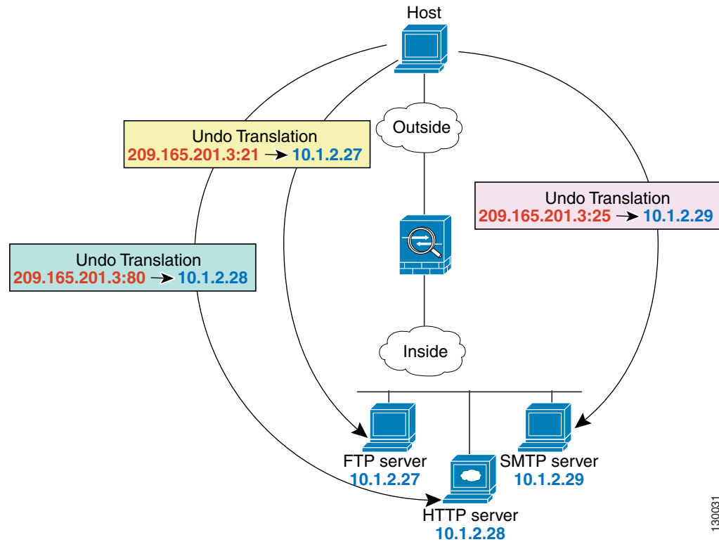
Figure 6-8 Static PAT
